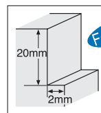
NC5-63 Material: S53C V=500m/min. f=0.25mm/tooth S=10000min -1 F=10000mm/min.
